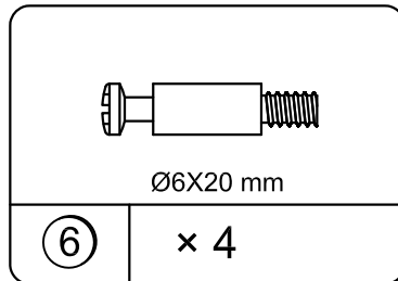
Cam bolt TKX1270
