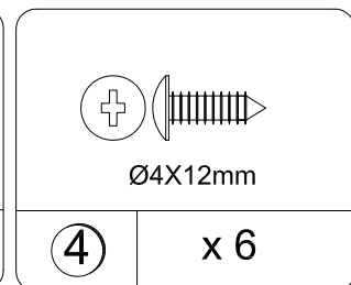
Screw TSF1004
